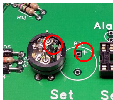
Figure 17 – BZ1 orientation [match the (+) marks]
