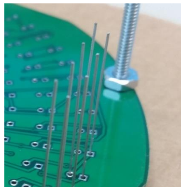
Figure 24 Long leads toward inside
