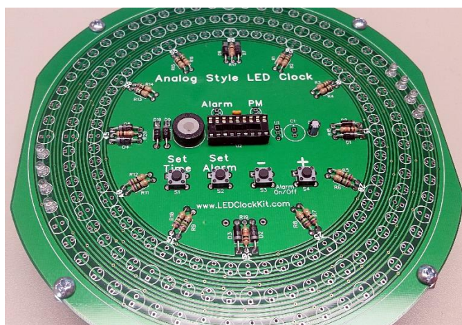
Figure 26 – Inserting LEDs eight at a time
