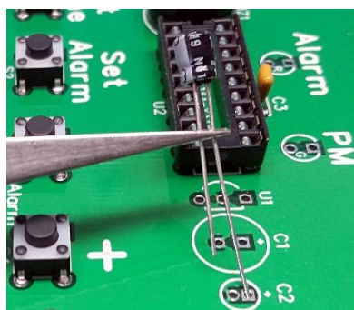
Figure 18 – C2 orientation
