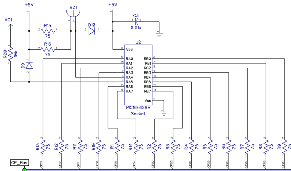
Figure 48 – Schematic, Microcontroller
