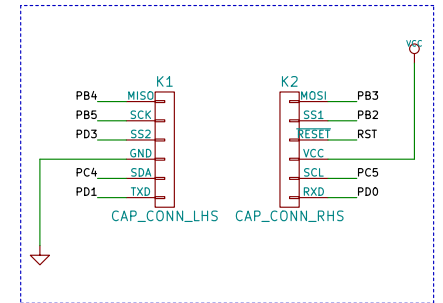
Common Cap Interface
